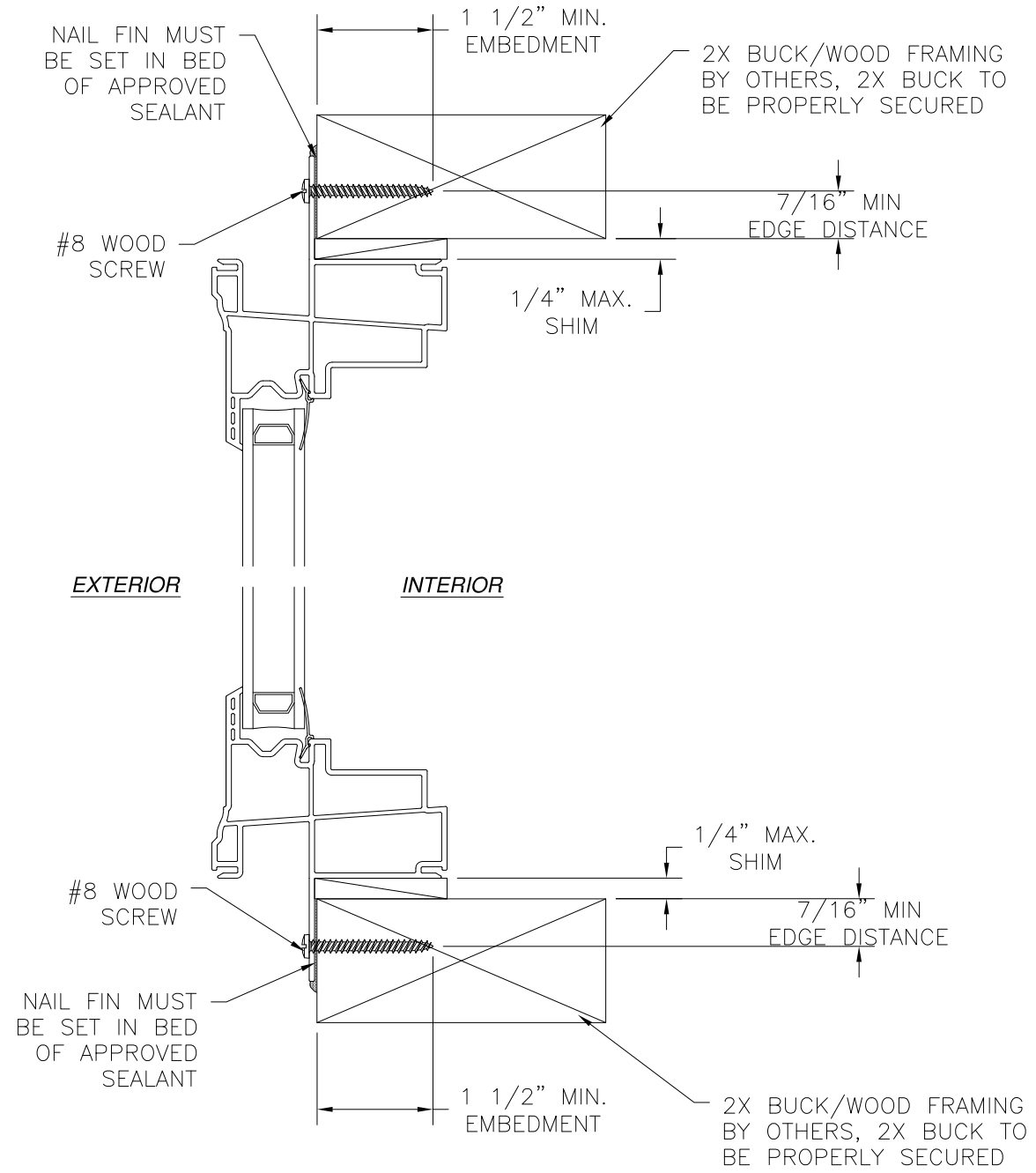
VERTICAL CROSS SECTION 2X BUCK/WOOD FRAMING INSTALLATION
