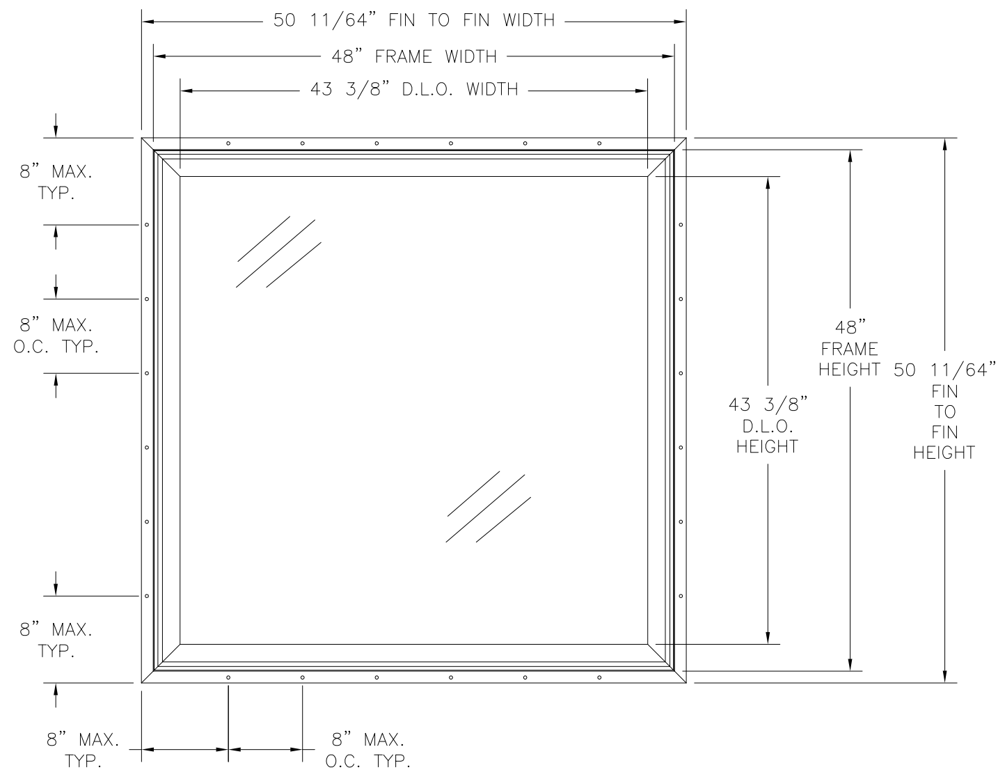
SHORELINE 1100 PW PVC FIXED PICTURE WINDOW EXTERIOR VIEW
